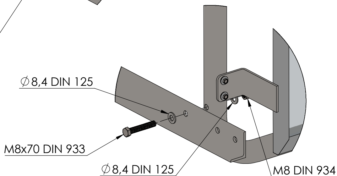
DETAIL I
