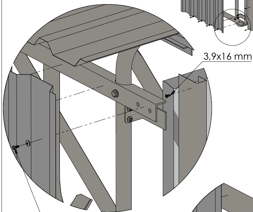
DETAIL J
