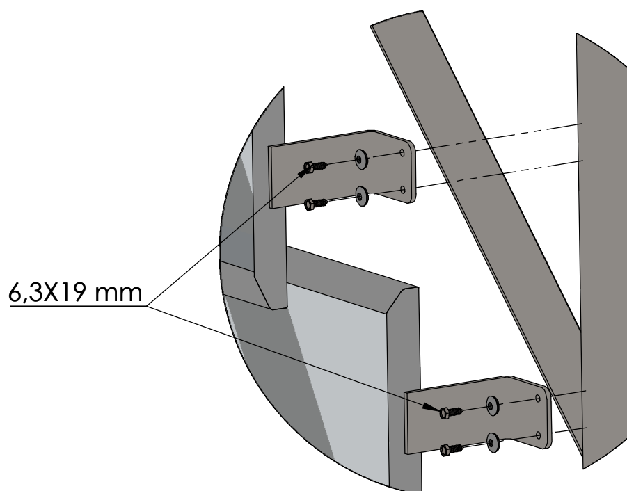
DETAIL G
