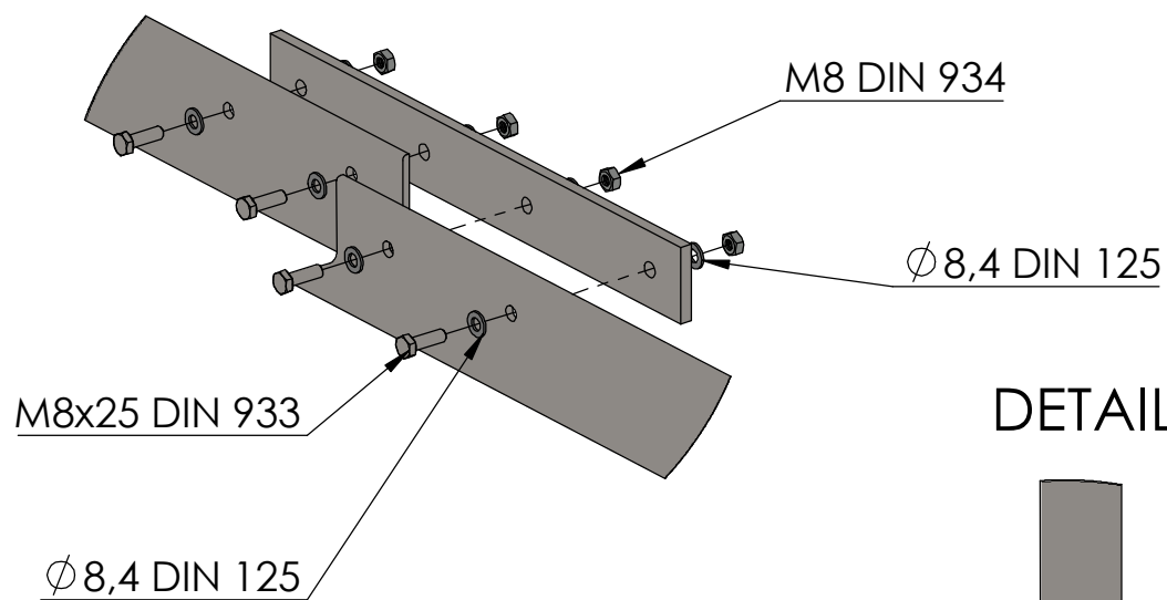
DETAIL H
