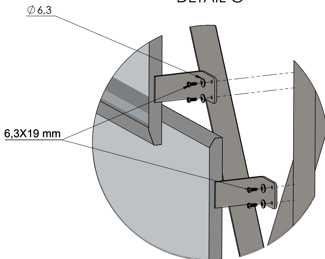
DETAIL G
