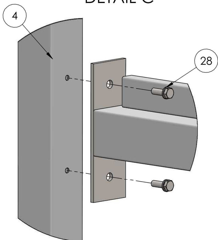
DETAIL C
