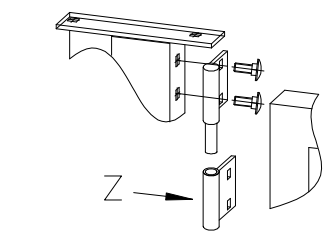
Detail W
